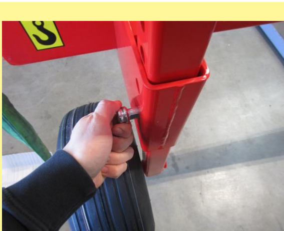
Figure 7: Inserting the feeler wheel and securing with the pin and linch pin.
